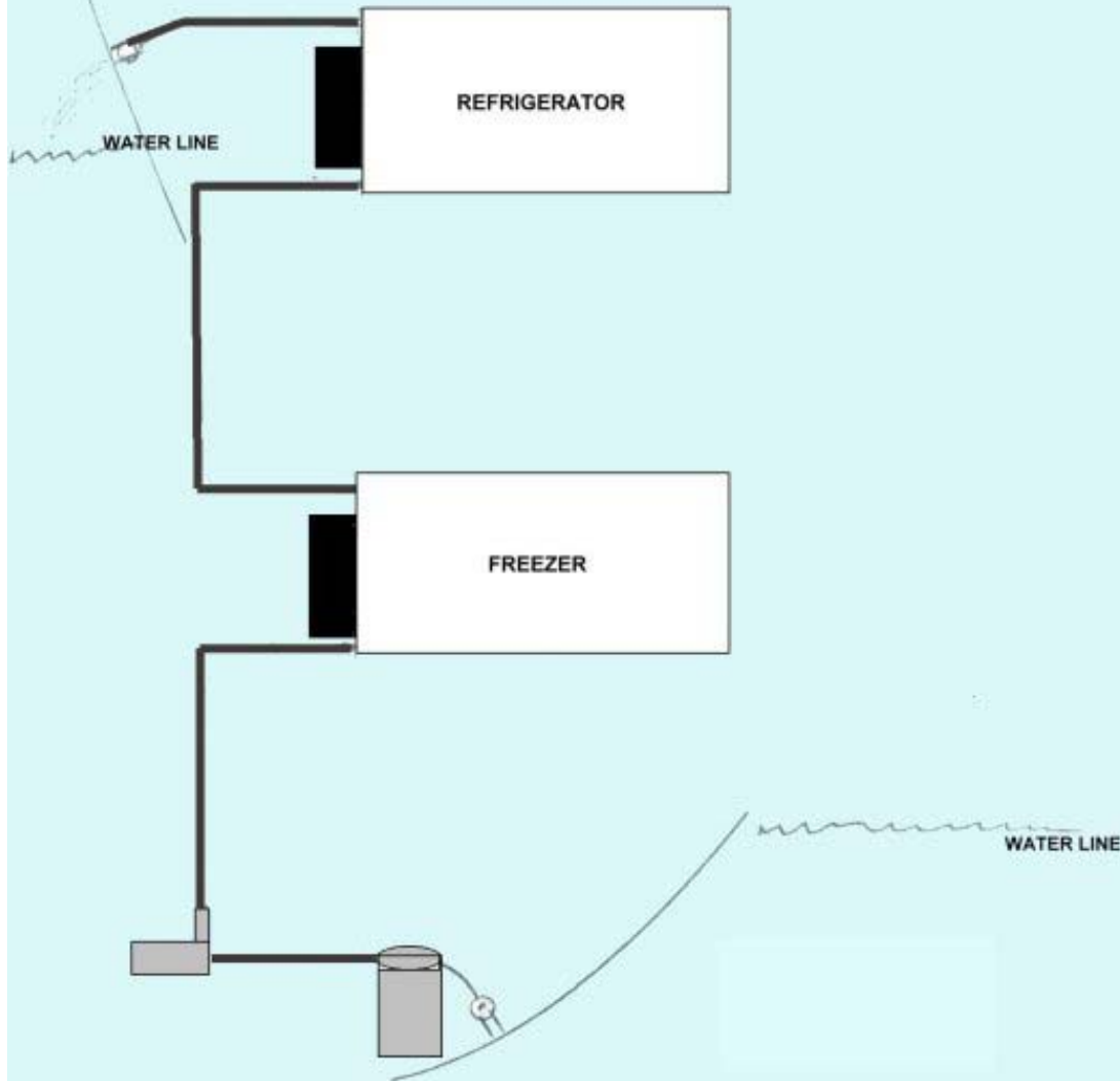
BD & Tradewinds Water Pump Wiring with Two Condensing Units
